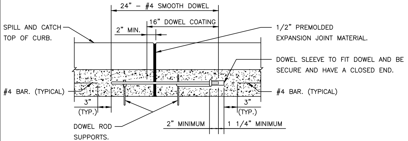
CURB EXPANSION JOINT DOWEL DETAIL
